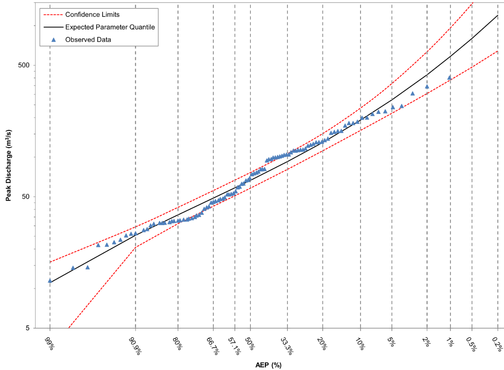
Figure D-3 FFA Results – GEV Distribution
