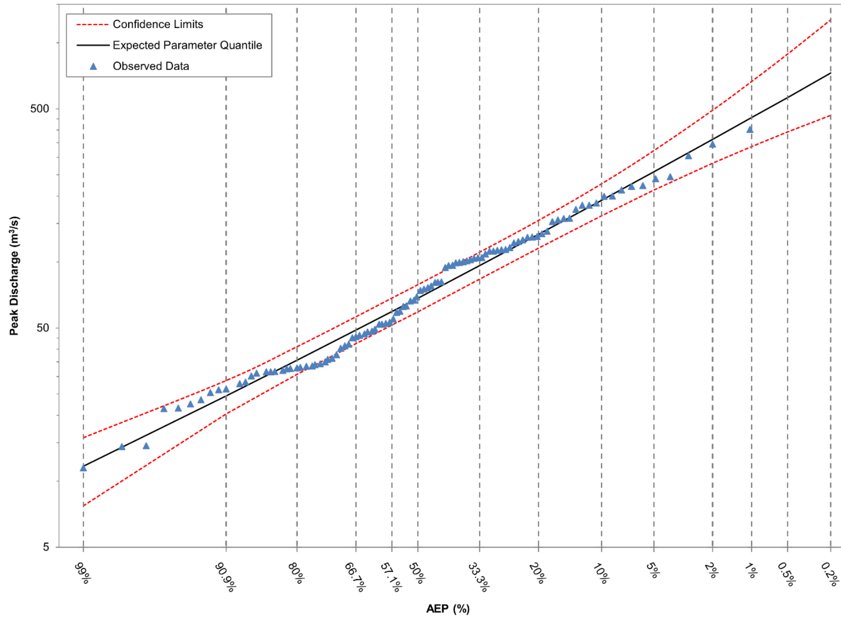
Figure D-1 FFA Results – LP3 Distribution
