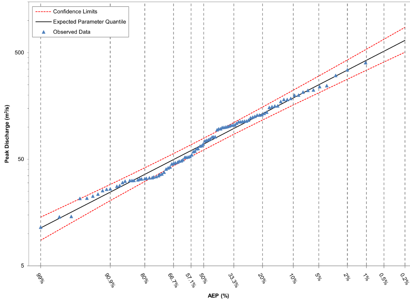
Figure D-2 FFA Results – Log-Normal Distribution
