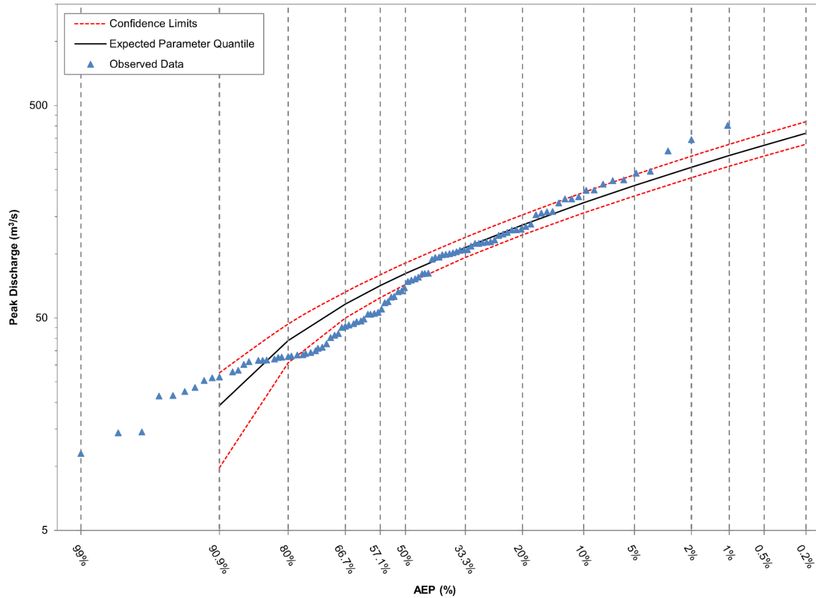
Figure D-4 FFA Results – Gumbel Distribution
